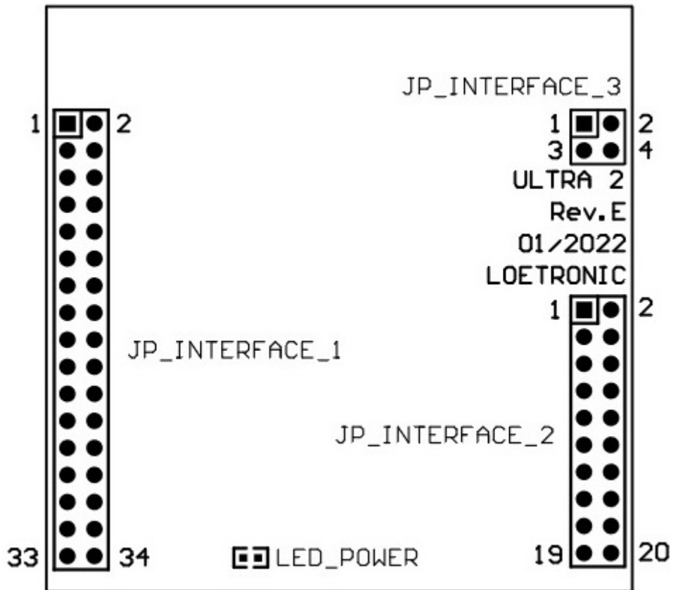
Picture 3.1 Fallguy ULTRA 2 MP3 module Rev.E – Connections
