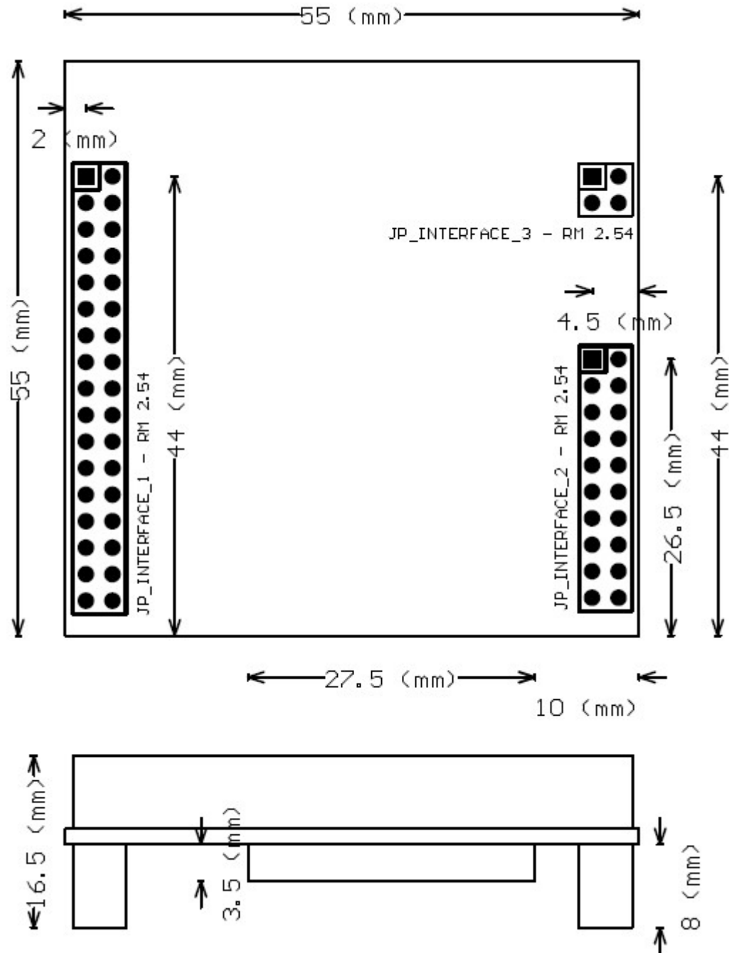
Picture 4.1 Fallguy ULTRA 2 MP3 module Rev.E - Dimensions
